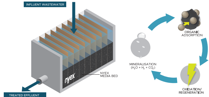
Figure 1 – Schematic of Arvia's Nyex™ Technology
