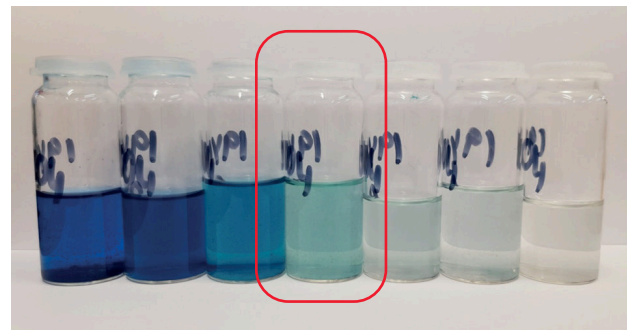
Figure 2: Colour removal results from Nyex-e system recirculation trial.
