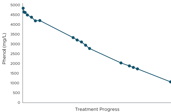
Figure 3. Sample 1: Phenol Removal from Chemical Distillate
