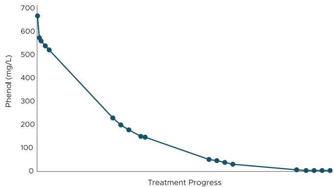
Figure 4. Sample 2: Phenol Removal from Chemical Effluent
