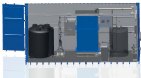
Containerised Nyex™ 7-100a Treatment System
