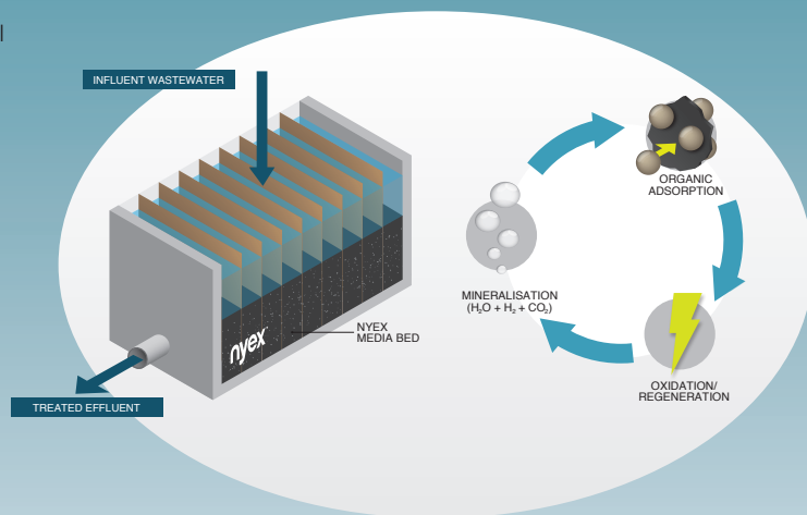
Figure 1 – Schematic of Arvia's Nyex™ Technology
