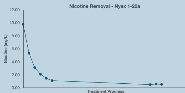
Figure 3 – Nicotine removal by Arvia's Nyex™ 1-20a system, against treatment progress
