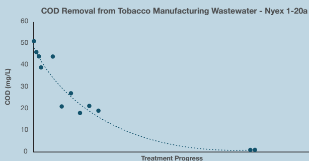
Figure 2 – On-site COD removal by Arvia's Nyex™ 1-20a system, against treatment progress
